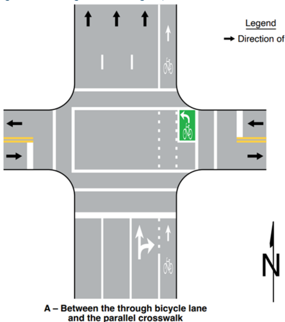
Figure 39: Two-Stage Turn Box Diagram, MUTCD
