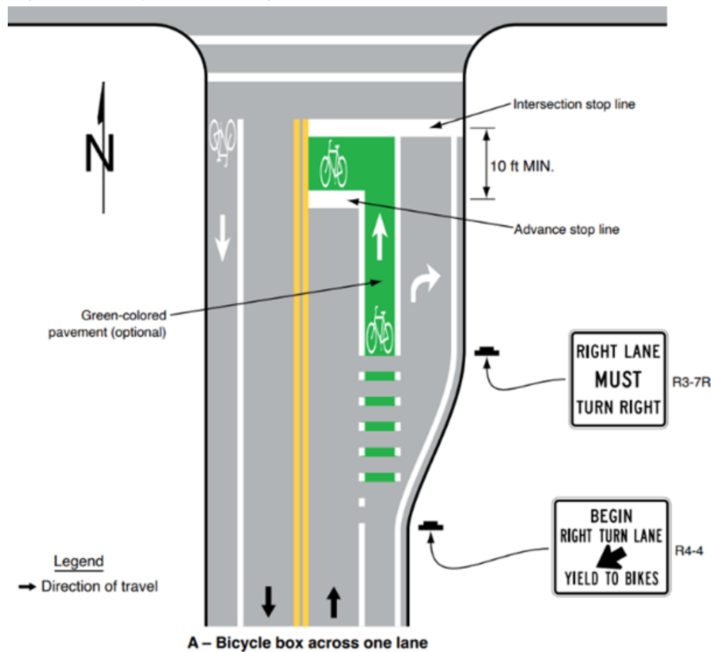
Figure 38: Bicycle Box Diagram, MUTCD
