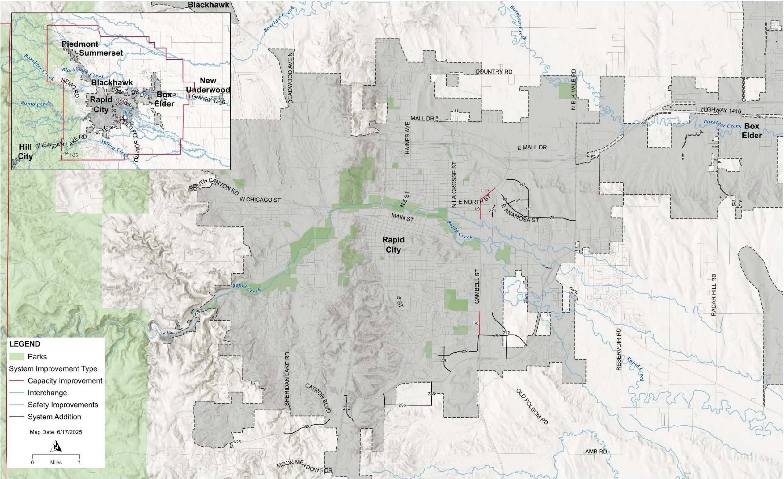
Figure 45: Mid-Term Roadway Improvements
