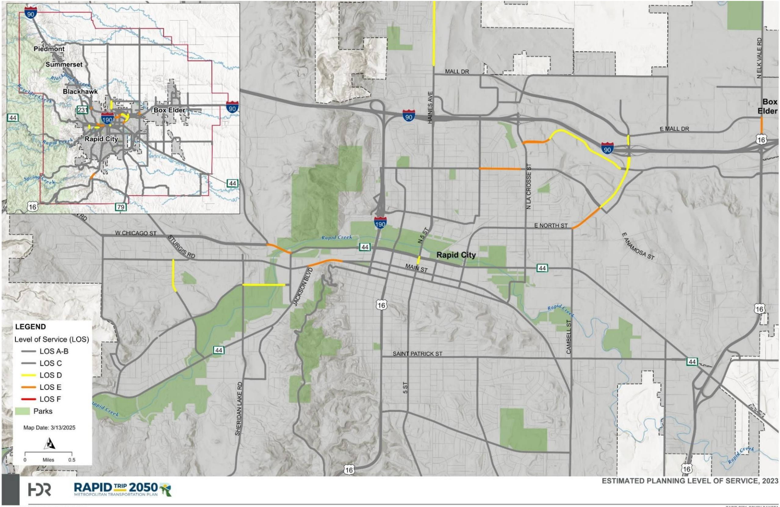
Figure 15: Estimated Planning Level of Service, 2023
