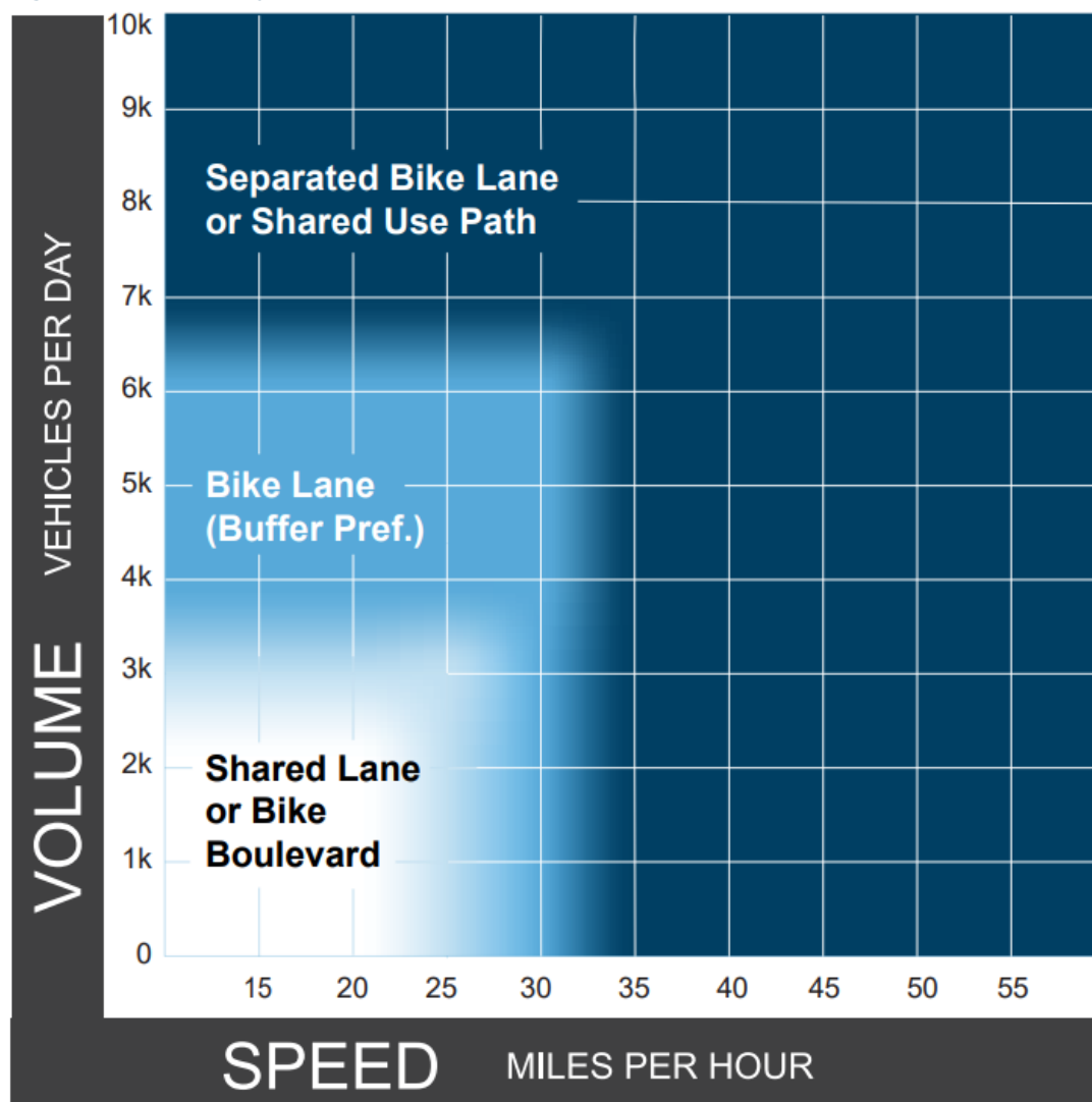
Figure 35: Bikeway Selection Guide
