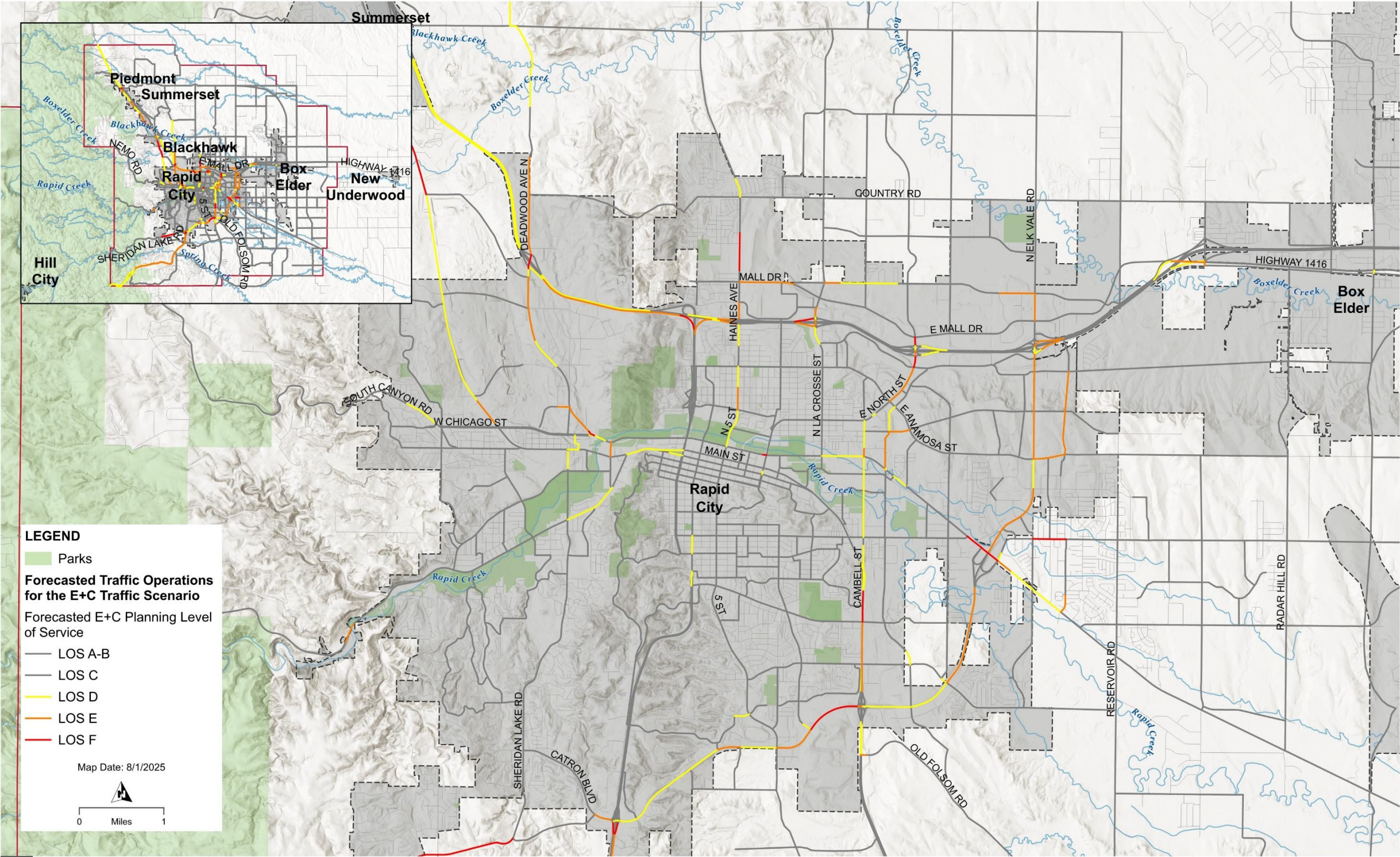
Figure 31: Forecasted Traffic Operations for the E+C Traffic Scenario
